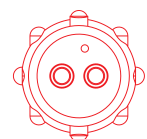
2 POSITION #20 PIN & SOCKET CONTACT
